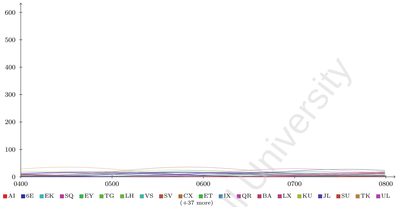
Figure 2: N6 entry-time density, composite overlay, 0400 to 0800 (4 h window).
