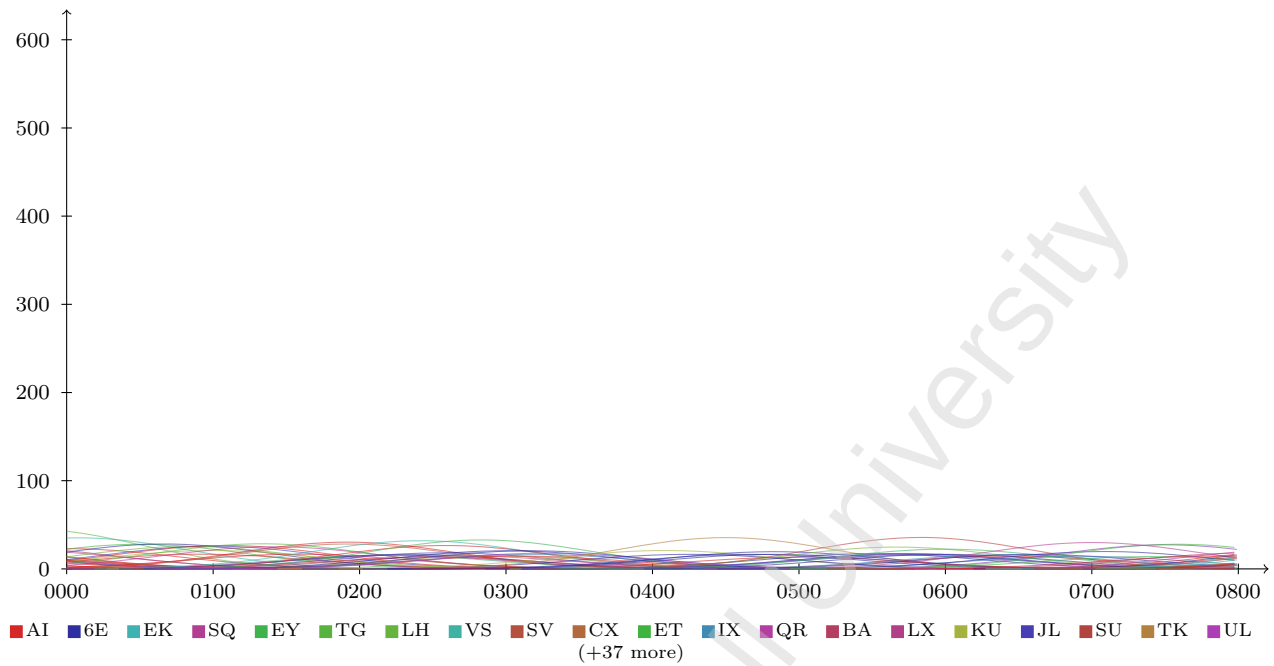
Figure 7: N6 entry-time density, composite overlay, 0000 to 0800 (8 h window).
