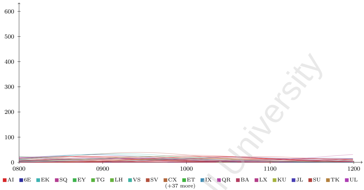
Figure 3: N6 entry-time density, composite overlay, 0800 to 1200 (4 h window).
