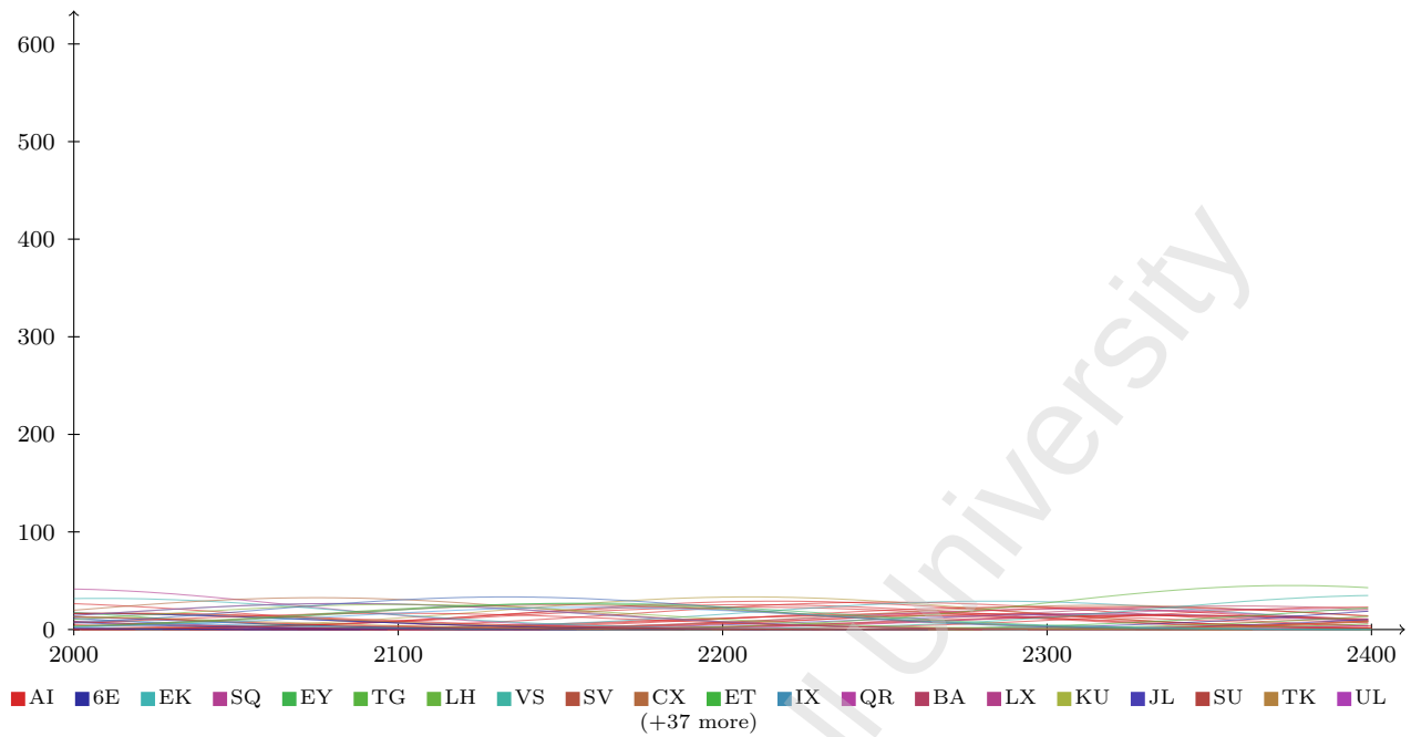
Figure 6: N6 entry-time density, composite overlay, 2000 to 2400 (4 h window).
