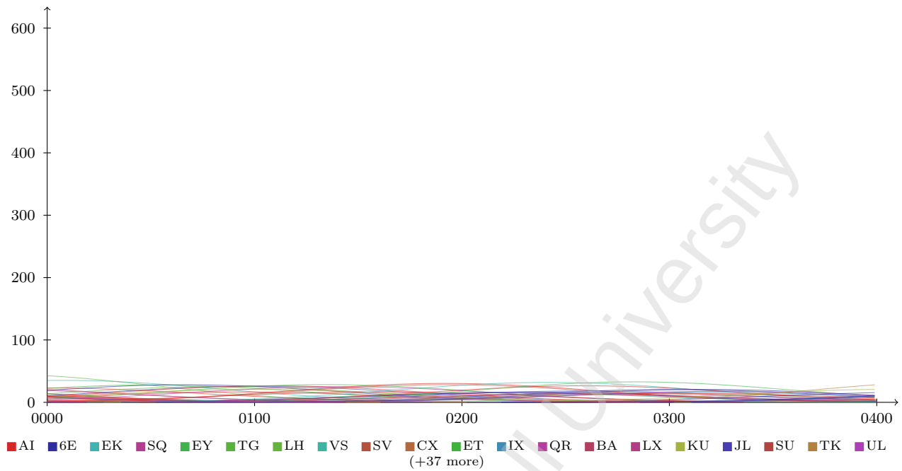
Figure 1: N6 entry-time density, composite overlay, 0000 to 0400 (4 h window).
