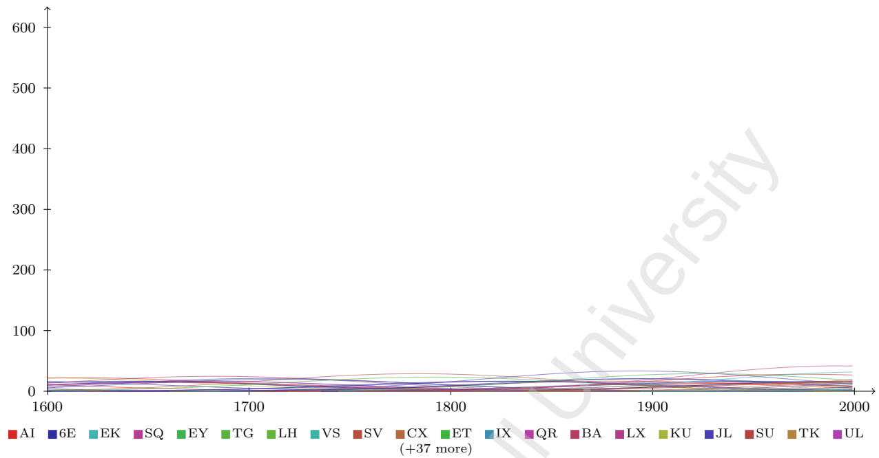
Figure 5: N6 entry-time density, composite overlay, 1600 to 2000 (4 h window).
