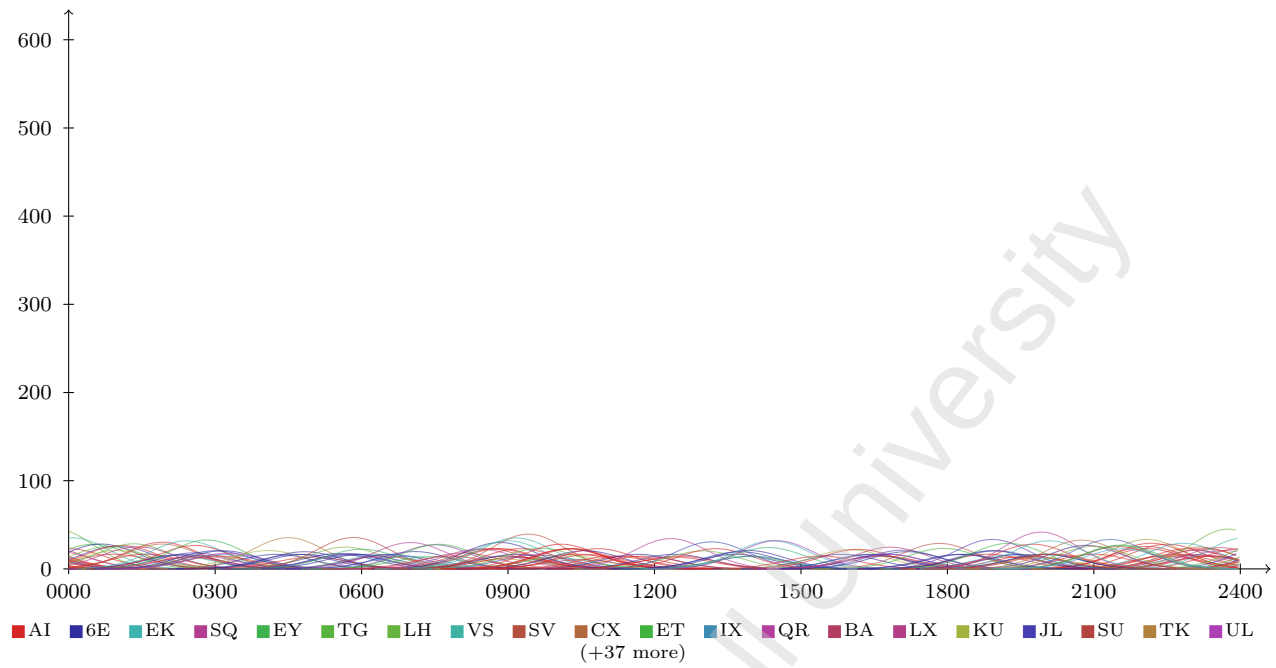
Figure 12: N6 entry-time density, composite overlay, 0000 to 2400 (24 h, full day).
